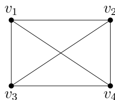
Fig:3-Complete graph K_4
